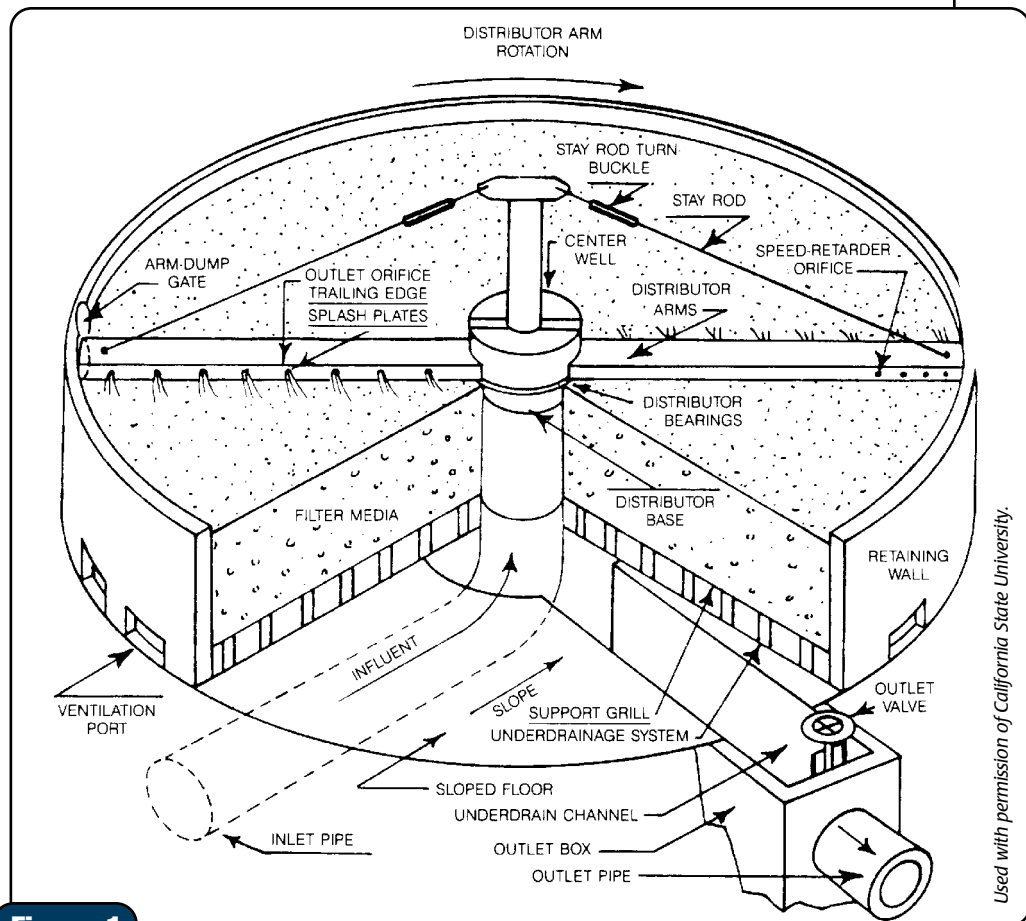
Figure 1 Parts of a typical trickling filter.
