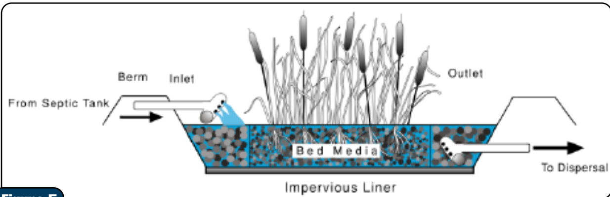
Figure 5 Constructed Wetland
