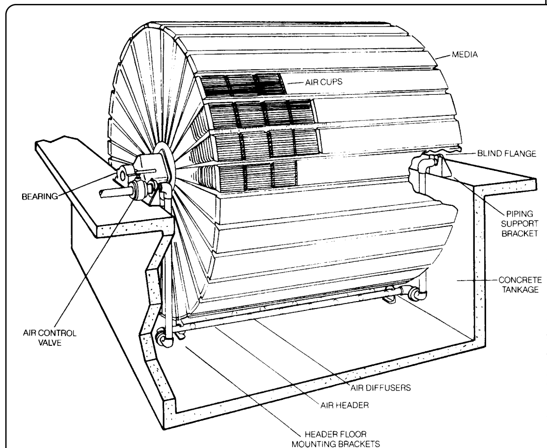
Figure 2 Rotating biological contactor
