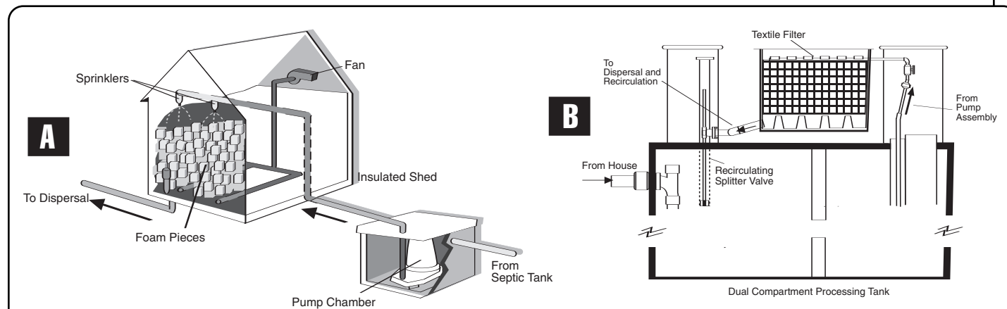
Figure 4 Foam Filters
