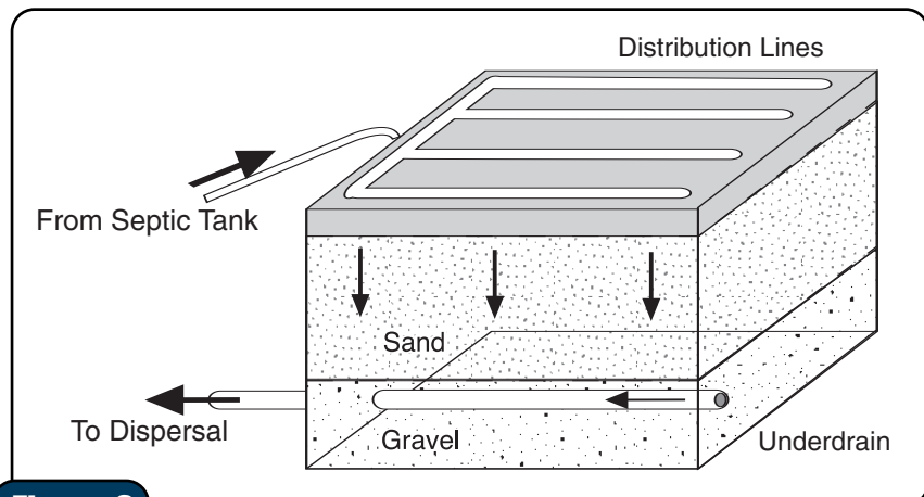
Figure 3 Sand Filter
