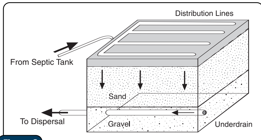
Figure 3 Sand Filter
